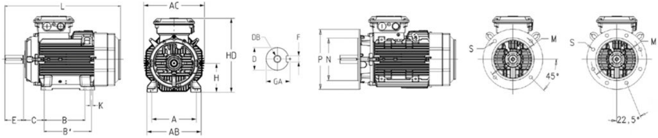
MAIN DIMENSIONS FOR HIGH OUTPUT SYNRM MOTORS (B-GENERATION)
