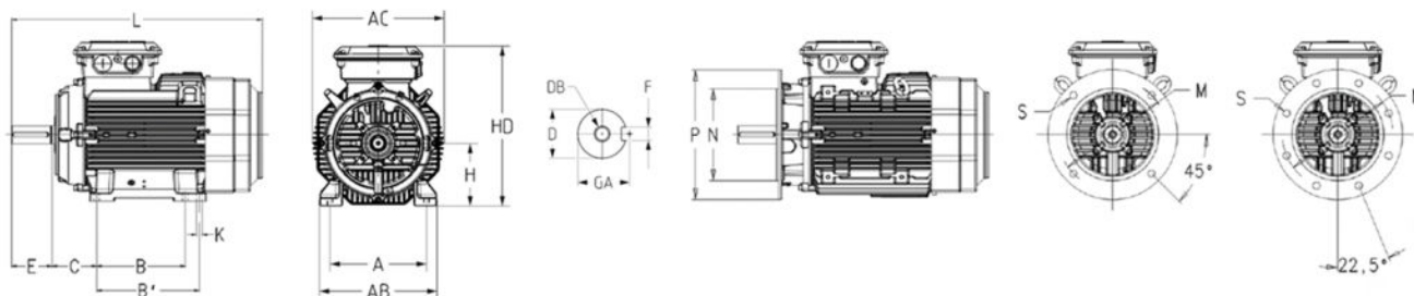
MAIN DIMENSIONS FOR IE5 SYNRM MOTORS (C-GENERATION)
